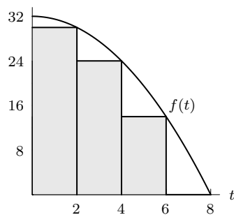
Figure 5.10: Right Sum, \Delta t = 2
