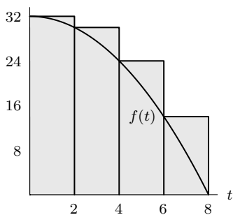
Figure 5.9: Left Sum, \Delta t = 2
