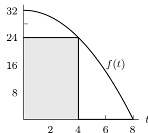
Figure 5.8: Right Sum, \Delta t = 4
