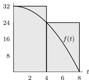
Figure 5.7: Left Sum, \Delta t = 4
