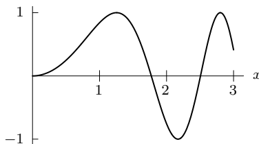
Figure 5.27: Graph of f'(x) = \sin(x^2)
