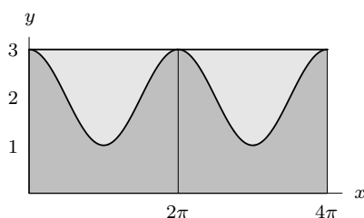
Figure 5.23: Integral vs. Left- and Right-Hand Sums
