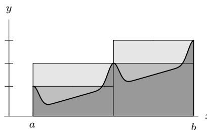
Figure 5.24: Integral vs. Left- and Right-Hand Sums
