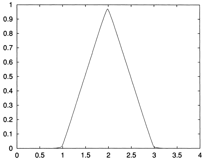
FIGURE 1. Graph of \phi_0 .
