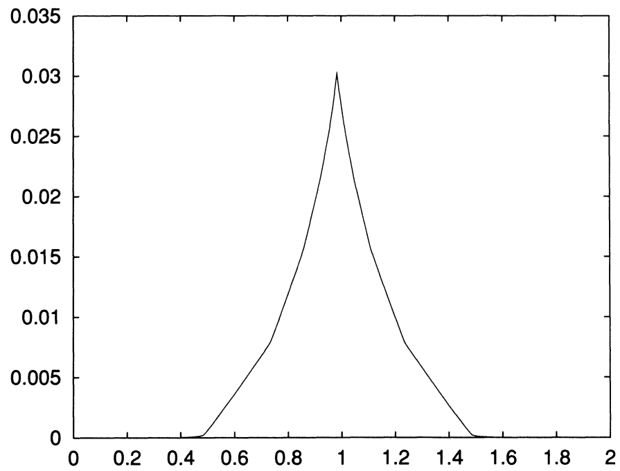
FIGURE 2. Graph of \phi_1 .
