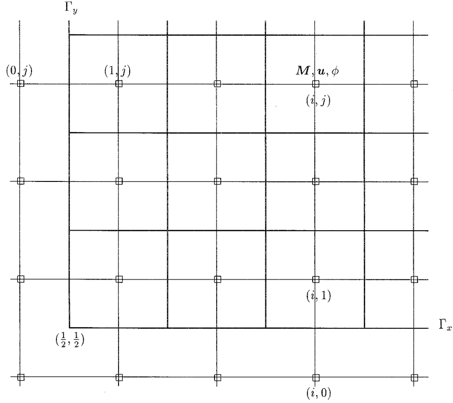
FIG. 7. Non-staggered grid.
