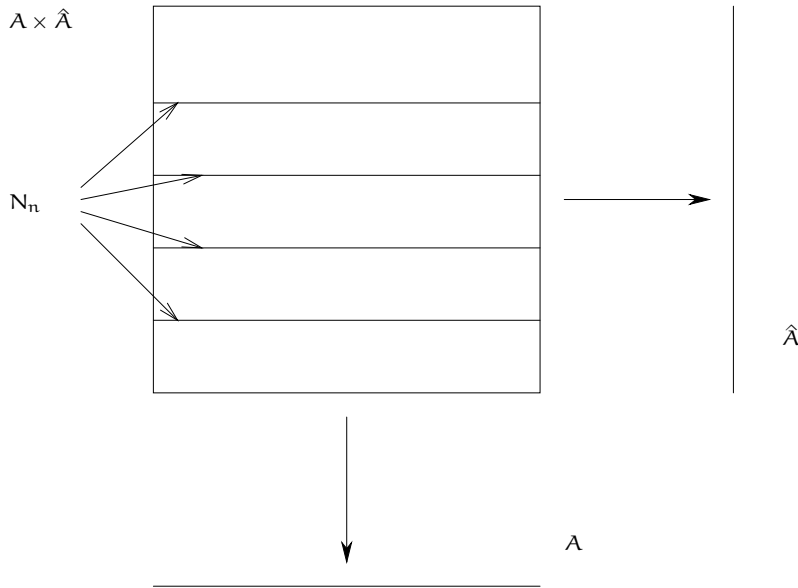
FIGURE 2. Factoring the universal cover of an abelian variety over k
