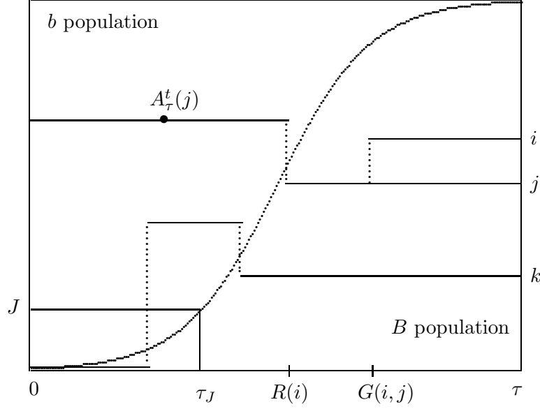
Figure 1. A picture to explain our notation. The lineages jump around as we move backwards in time, but for simplicity we have only indicated the recombination events. Here as we work backwards in time i and j coalesce and then recombine into the b population. Proposition 2.4 shows that this event has probability at most C/\log N . Proposition 2.1 estimates the probability of two recobminations as shown in lineage k .
