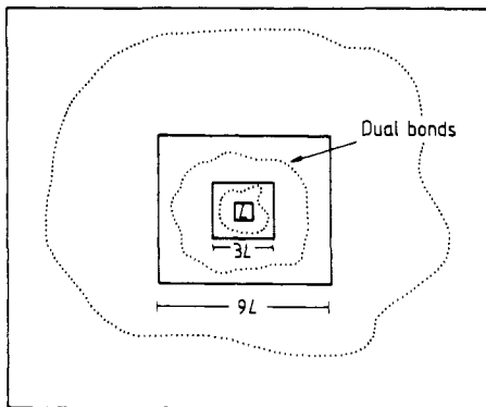
Figure 2. Circuits in annuli.
